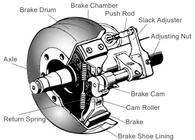
Figure 5-2: S-cam Drum Brake
